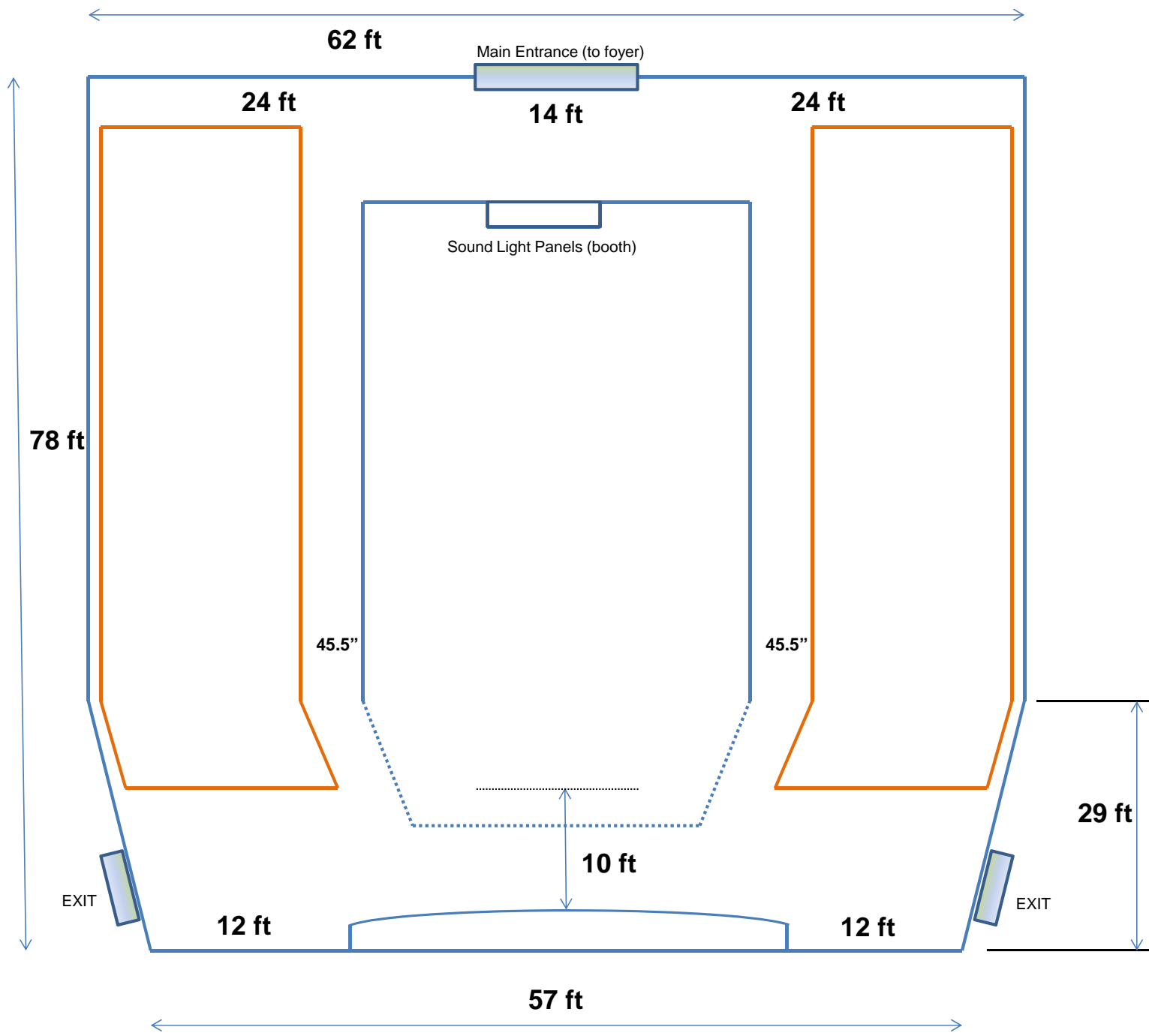
Floor Plans Bronson Centre Theatre 2016 - Main
